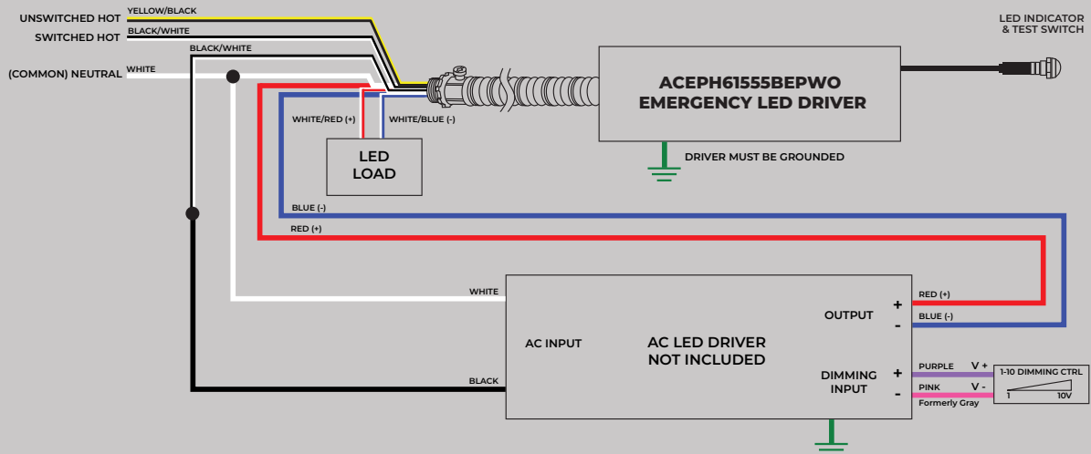
A. TYPICAL WIRING DIAGRAM FOR SWITCHING THE SWITCHED HOT AC POWER FOR THE NORMAL AC LED DRIVER
