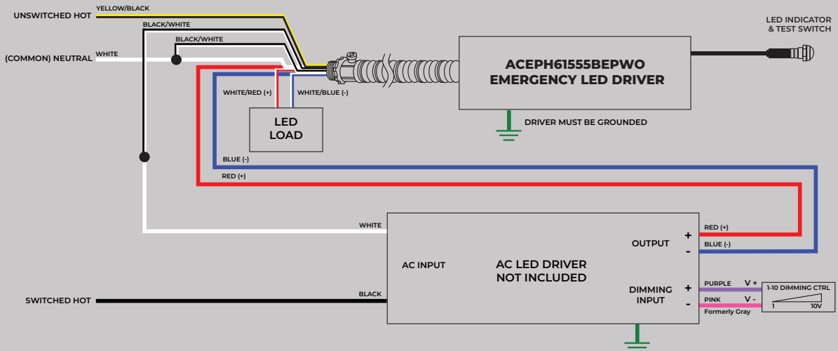
B. TYPICAL WIRING DIAGRAM FOR SWITCHING THE NEUTRAL WIRE OF THE NORMAL AC LED DRIVER
