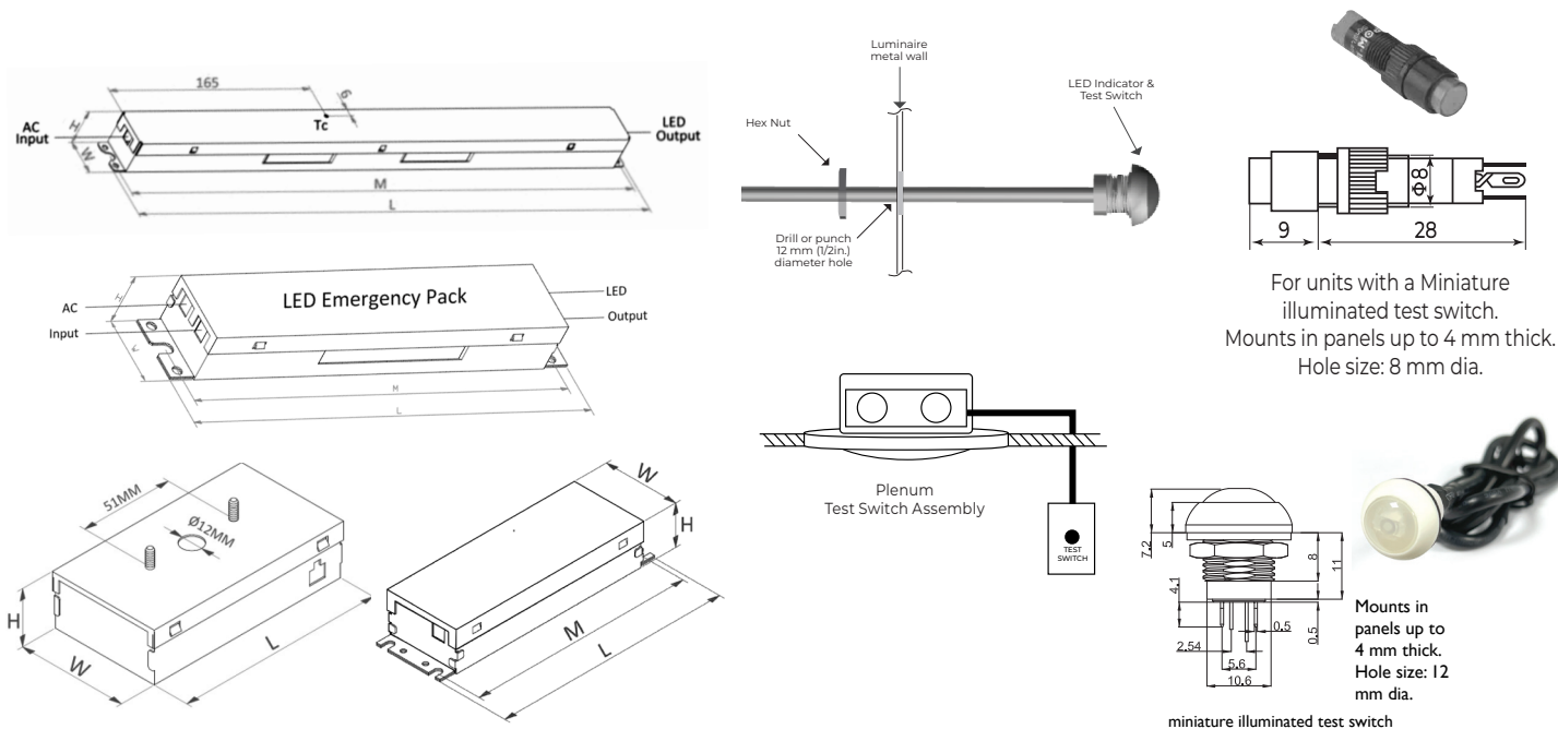
Illustration 1. See the individual product specifications for unit dimensions, location of Tc, and mounting tabs
