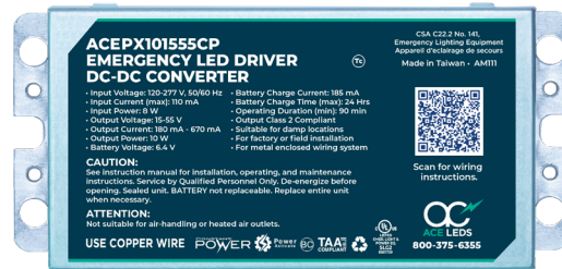
DC-DC CONVERTER
