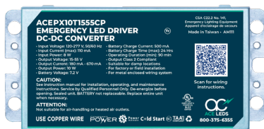
DC-DC CONVERTER
