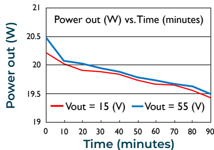
Constant output power performance over full 90 minutes run-time
