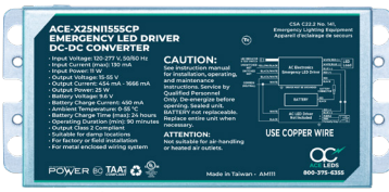
DC-DC CONVERTER
