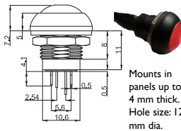
miniature illuminated test switch
