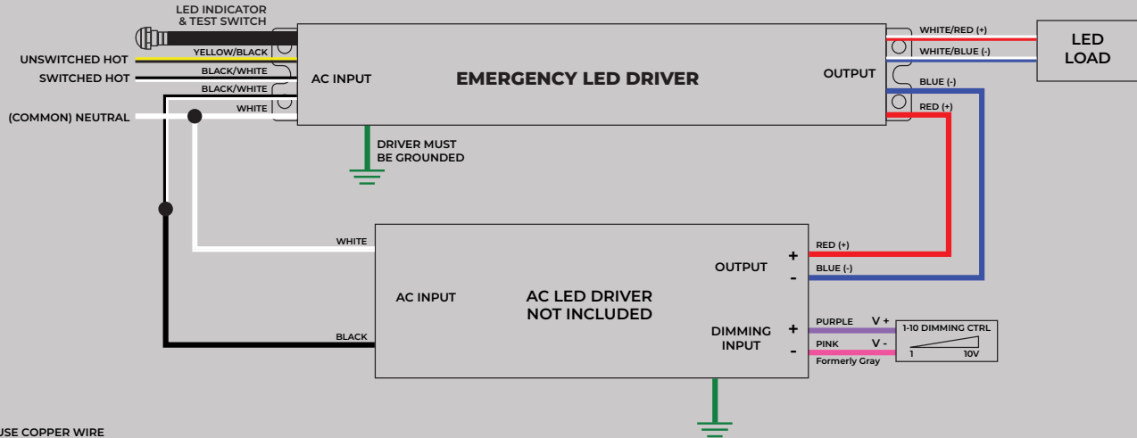
A. TYPICAL WIRING DIAGRAM FOR SWITCHING THE SWITCHED HOT AC POWER FOR THE NORMAL AC LED DRIVER
