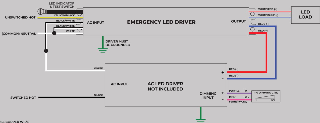
B. TYPICAL WIRING DIAGRAM FOR SWITCHING THE NEUTRAL WIRE OF THE NORMAL AC LED DRIVER
