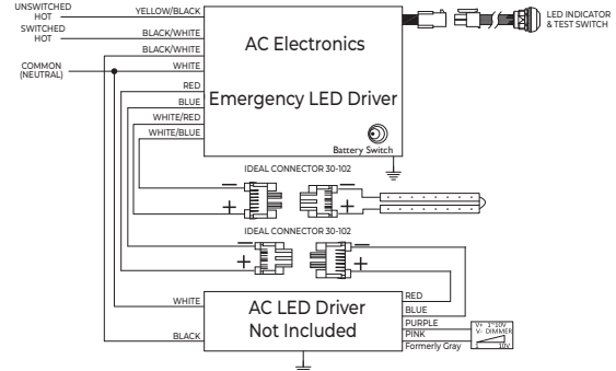
WIRING DIAGRAM FOR SWITCHING THE SWITCHED HOT AC POWER FOR THE NORMAL AC LED DRIVER
