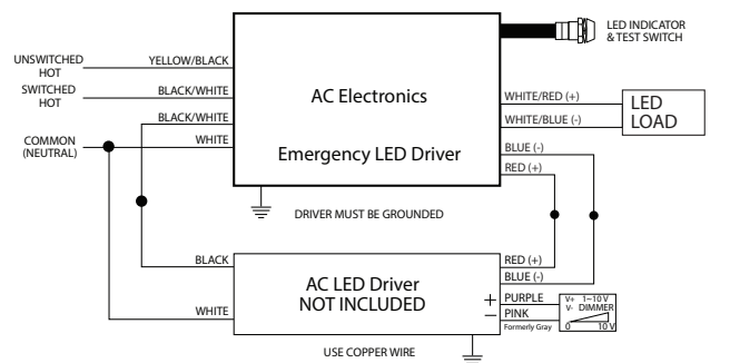
WIRING DIAGRAM FOR SWITCHING THE SWITCHED HOT AC POWER FOR THE NORMAL AC LED DRIVER
