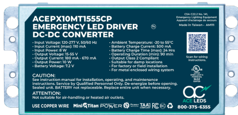
DC-DC CONVERTER
